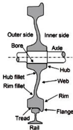
Figure 2. Designation of each part of solid wheel [1]
