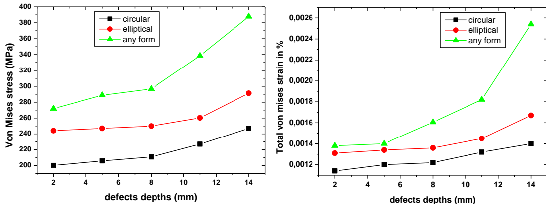
Figure 9. Varying the Von Mises Stress and the total Von Mises Strain versus depth of defects
