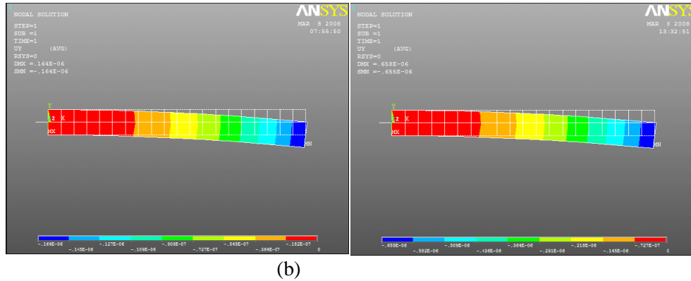
FIGURE 5. Deformation of bimorph beam actuated by electrical extensions: (a) 50 volts (b) 200 volts
