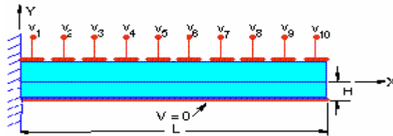
FIGURE. 4. Geometry of the embedded-free piezoelectric beam (L = 10mm, H = 0.25mm).
